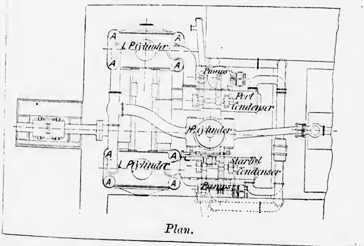
THREE CYLINDER COMPOUND ENGINES, MONTANA AND DAKOTA, 1872.
